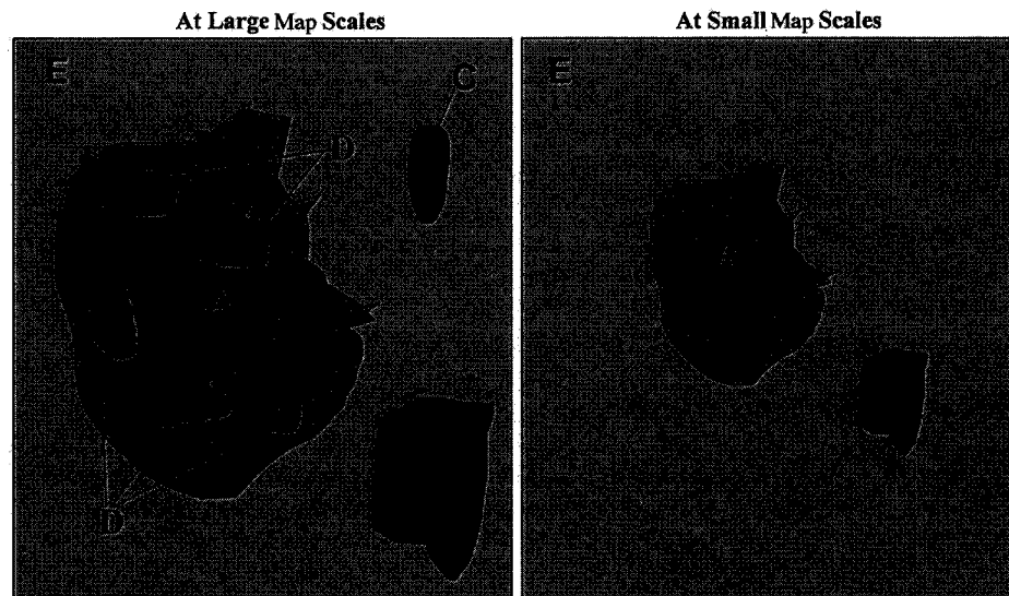
Fig. 5. Representation of soil bodies at different scales. Soil unit D and C on large-scale soil maps will disappear or be merged into soil unit A on small-scale soil maps.
