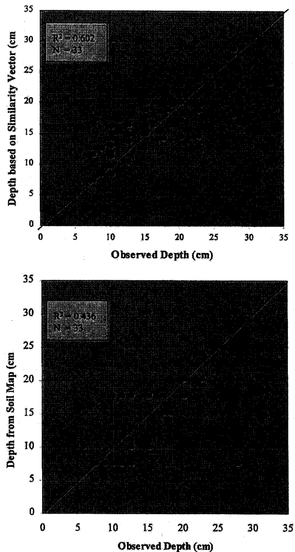
Fig. 11. Scatter plot of the depths based on the similarity vectors vs. observed depths (top) and that of the depths from the soil map vs. observed depths (bottom) for the 33 field sites.
